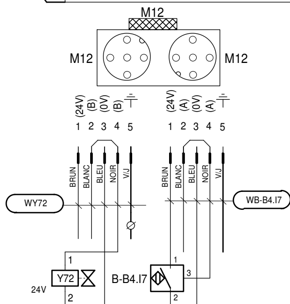
EV SELECTION OUTIL 3 POINCONNEUSE
